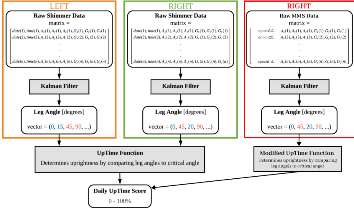
Figure 1.3: Left: UpTime calculation workflow with Shimmer (Palombo [15], Figure 3.5, Appendix E). Right: Modified UpTime calculation workflow with MMS (Appendix A).
