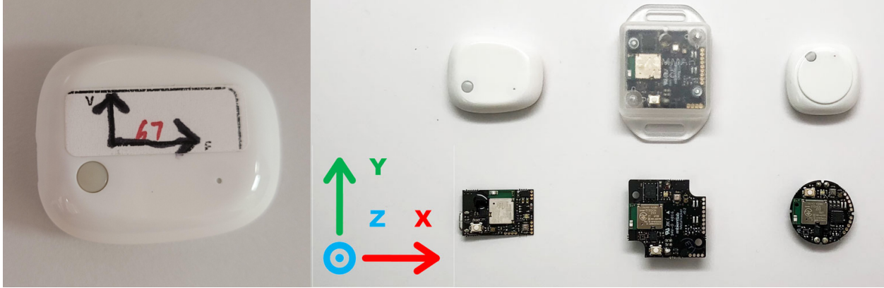
Figure 1.4: Left: one of our MMS in use, f means “forward”, v means “vertical”, during deployment, MMS devices are worn on study participants’ lower right leg, on the outer side of ankle, with the label facing outward. Right: official Bosch BMI160 6-axis IMU orientation labeling from MbiEntLab, image source: https://mbientlab.com/tutorials/Orientation.html .
